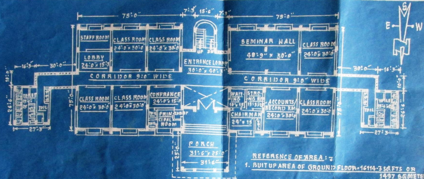
GROUND FLOOR PLAN SCALE:- 1" = 20' FTS.
